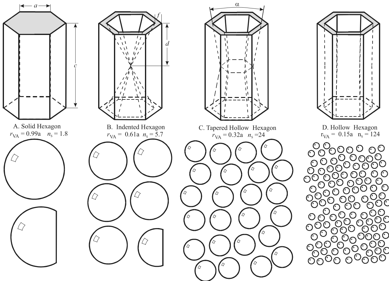
Figure 2. Geometry of the hollow hexagons and associated equal- V/A spheres for a given value of the half-width of the basal face, a . The crystal length is c , the depth of the indentation is d , and the basal shoulder width is f . In terms of the ratios defined in equations (3)–(5), the crystals shown are specified as follows: (a) \Gamma = 1.4 , \Psi = 0 , \alpha = 180^\circ ; (b) \Gamma = 1.4 , \Psi = 1.0 , \Phi = 0.2 , \alpha = 60^\circ ; (c) \Gamma = 1.4 , \Psi = 3.0 , \Phi = 0.2 , \alpha = 20^\circ ; and (d) \Gamma = 1.4 , \Psi = 100 , \Phi = 0.2 , \alpha \approx 0^\circ , where \alpha is the opening angle as shown in Figure 2c. The corresponding size and number of equal- V/A spheres are given below each crystal. The opening angle, \alpha , is given by \alpha = 2 \tan^{-1}[(1 - \Phi)/(\Gamma\Psi)] .
